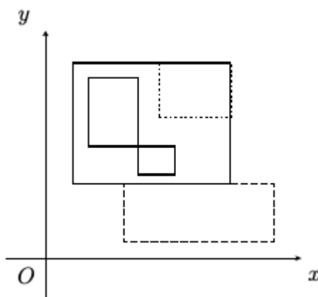
Figure C.2. Rectangles overlapping in more complex ways. This corresponds to the second dataset.
