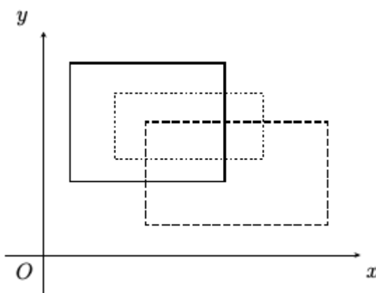
Figure C.1. Three rectangles partition the plane into eight regions. This corresponds to the first dataset of the sample input. The x - and y -axes are shown for illustration purposes only, and therefore they do not partition the plane.
