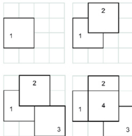
Fig 1. Placing four filled squares in an empty 4 \times 4 grid.
