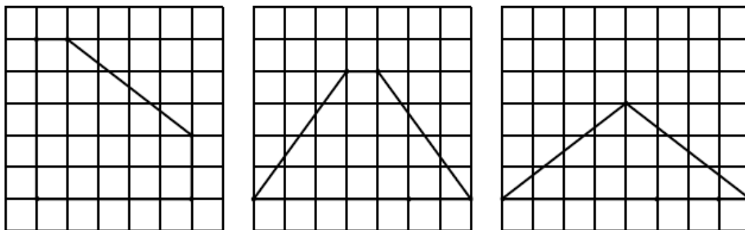
Figure 7: Convex polygons consisting of five rods of lengths 1, 2, 5, 5, and 5
