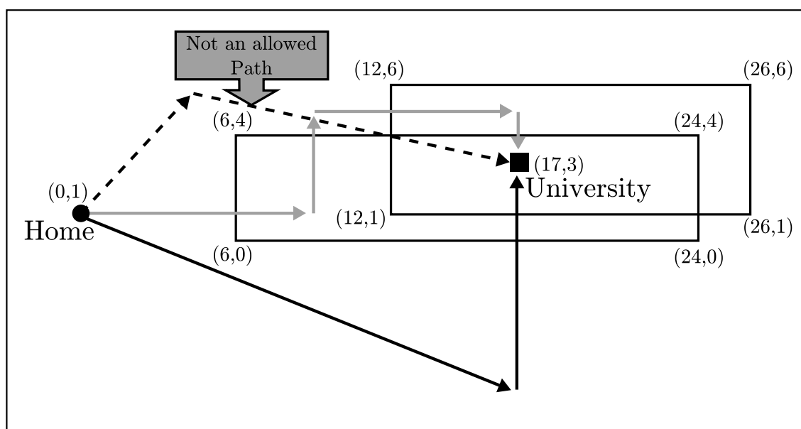
Figure: Streets are shown as straight lines and the arrows show possible walking paths for Peter. The black arrows show one possible path for Peter where he only has to cross two streets. The gray arrows show a path for Peter where he needs to cross four streets. The path shown by the dotted arrows is not legal because it crosses two streets at an intersection. The figure above corresponds to the first sample input.
